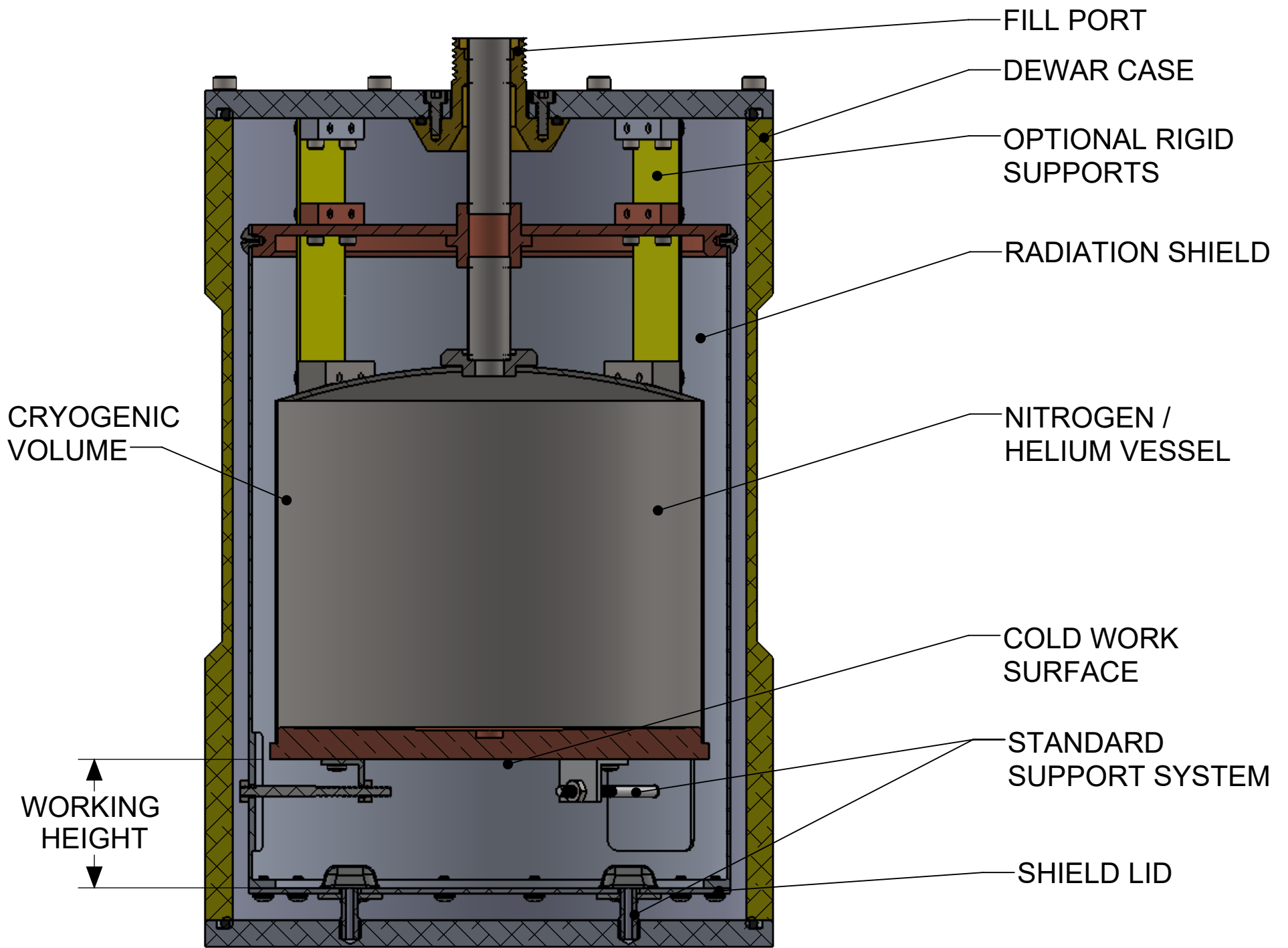
SECTION C-C
